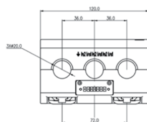
DR3N1-160/5A - 250/5A
